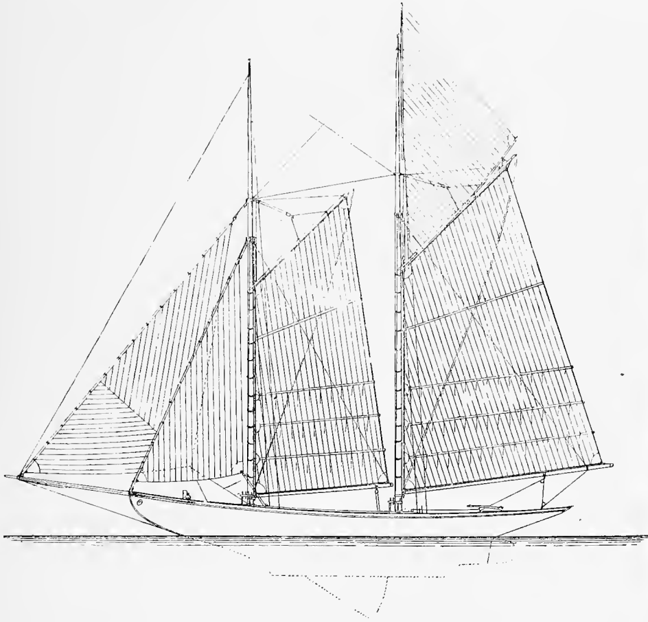
SAIL PLAN OF RICHARD P. JOY'S SCHOONER YACHT PILOT.
